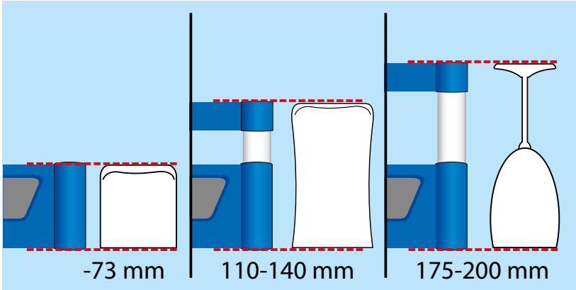
Glass heights for all basket sets with shallow top frame: • Max. 73 mm without extenders and without top frame • 110–140 mm with short extenders* • 175–200 mm with long extenders*
